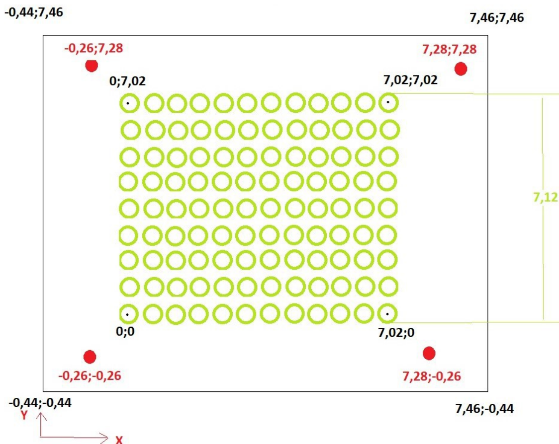
Figure 4. Back Light L4040 Dimensions
