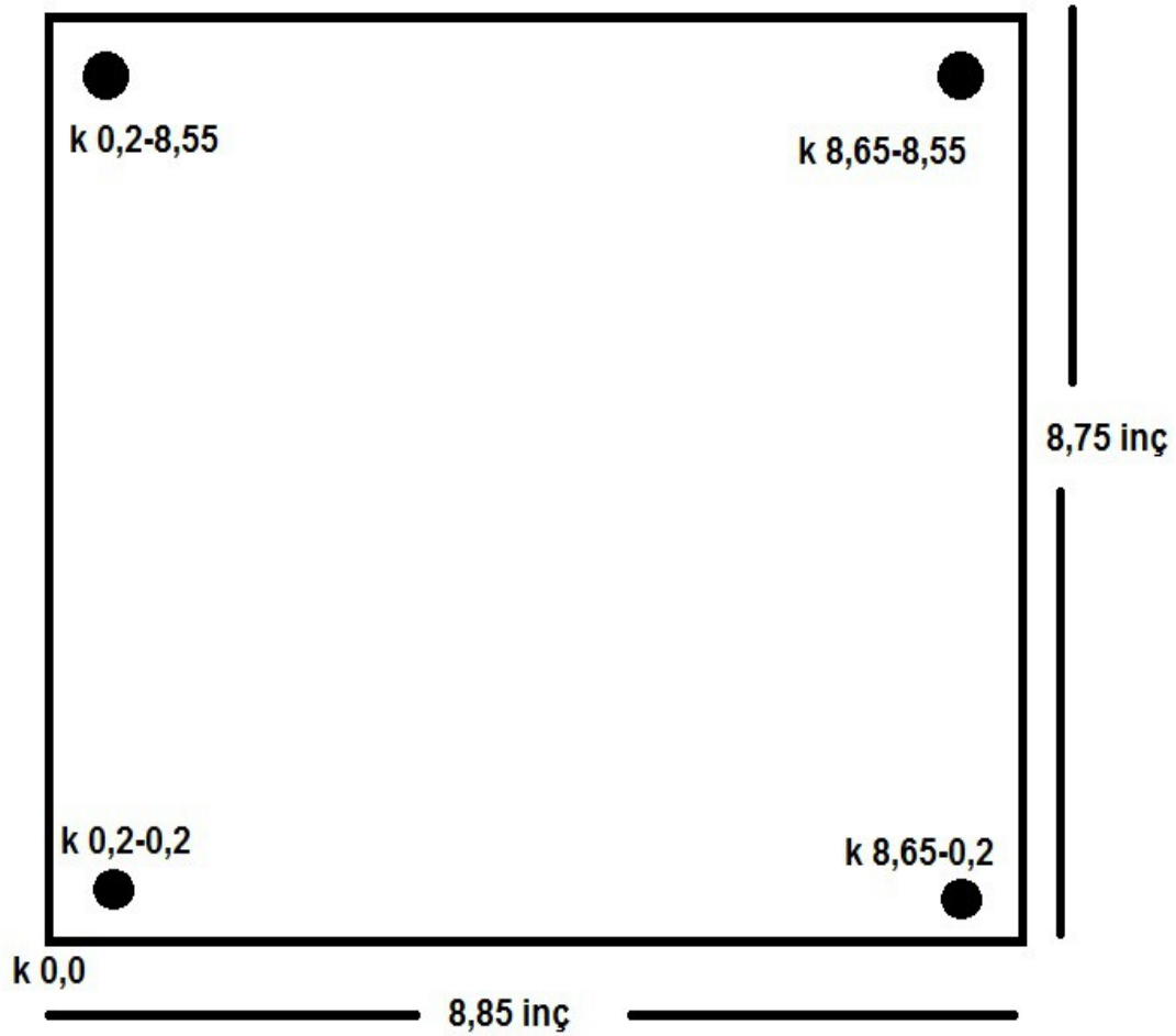
Figure 4. Back Light L3232 Dimensions
