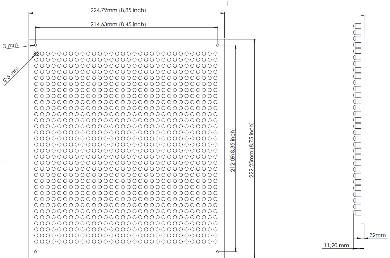
Figure 4.2. Back Light L3232 Dimensions
