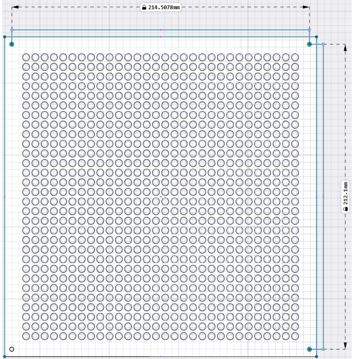
Figure 4.1. Back Light L3232 Mounting Hole Dimensions
